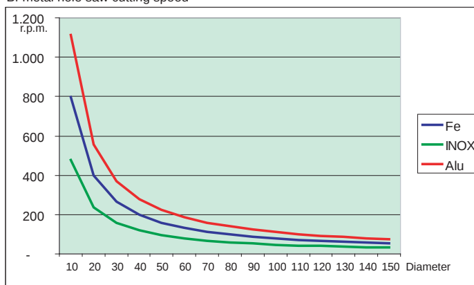
Bi-metal hole saw cutting speed
