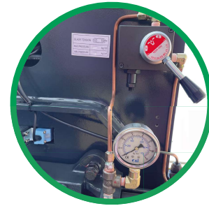
HYDRAULIC BELT TENSIONING DEVICE
