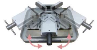
Radially and diagonally adjustable
